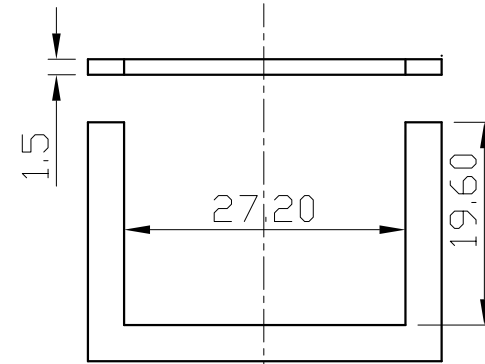
PANEL CUT-OUT
